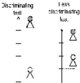
Two tests of varying discrimination
