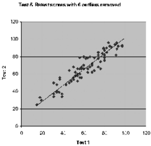
CB BULATS ability scores compared in two sittings
