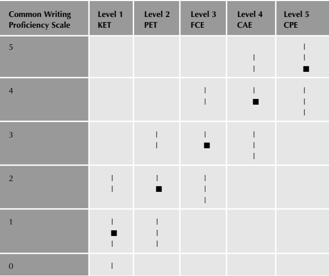
A common scale across examination levels and ranges
